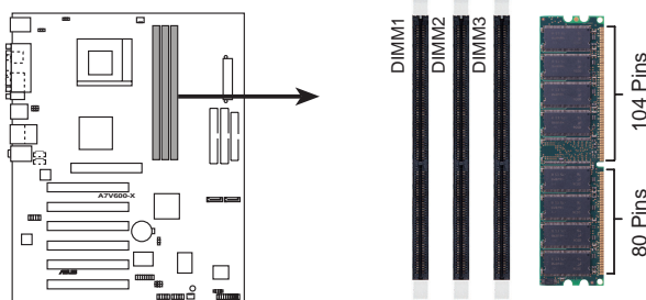
A7V600-X 184-Pin DDR DIMM Sockets
