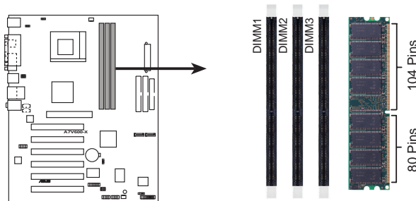
A7V600-X 184-Pin DDR DIMM Sockets
